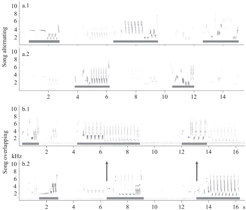
FIG. 1. Sound spectrograms from two vocal interactions in male nightingales, exemplifying song alternating (a.1 and a.2) and song overlapping (b.1 and b.2). Overlapping events are marked with arrows and the duration of a song is highlighted by gray bars below each song. Songs from interacting individuals are faintly visible also in the spectrogram of songs from its counterpart.
