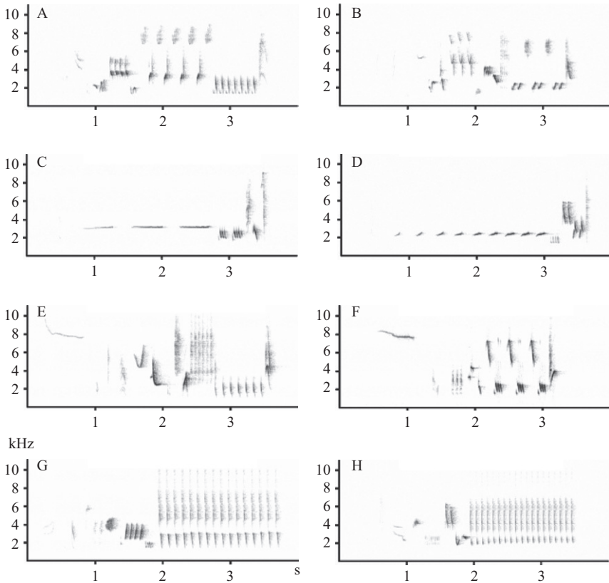
FIG. 2. Sound spectrograms nightingale songs with different structural components. (A) and (B) represent ordinary nightingale songs; (C) and (D) represent whistle songs, characterized by the series of whistles in the first part of the song; (E) and (F) represent songs preceded by initial whistles which are higher in frequency and lower in volume than the whistle in whistle songs. They also are usually not repeated within a song but often precede subsequent ordinary songs; (G) and (H) represent songs containing rapid broadband trills.
